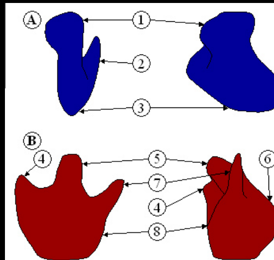
Figure 1 : The subunits of a ribosome. Side and front view.
