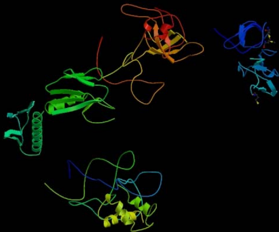
5 Å Map Of The Large Ribosomal Subunit
